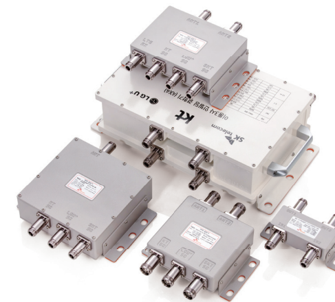
3 Combiners
